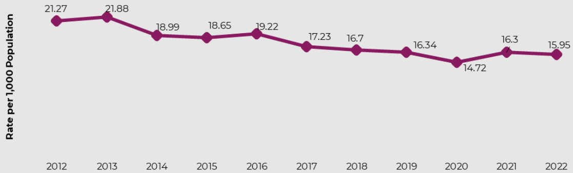
Figure 2 Annualized property crime rate mid-year 2012-2022
